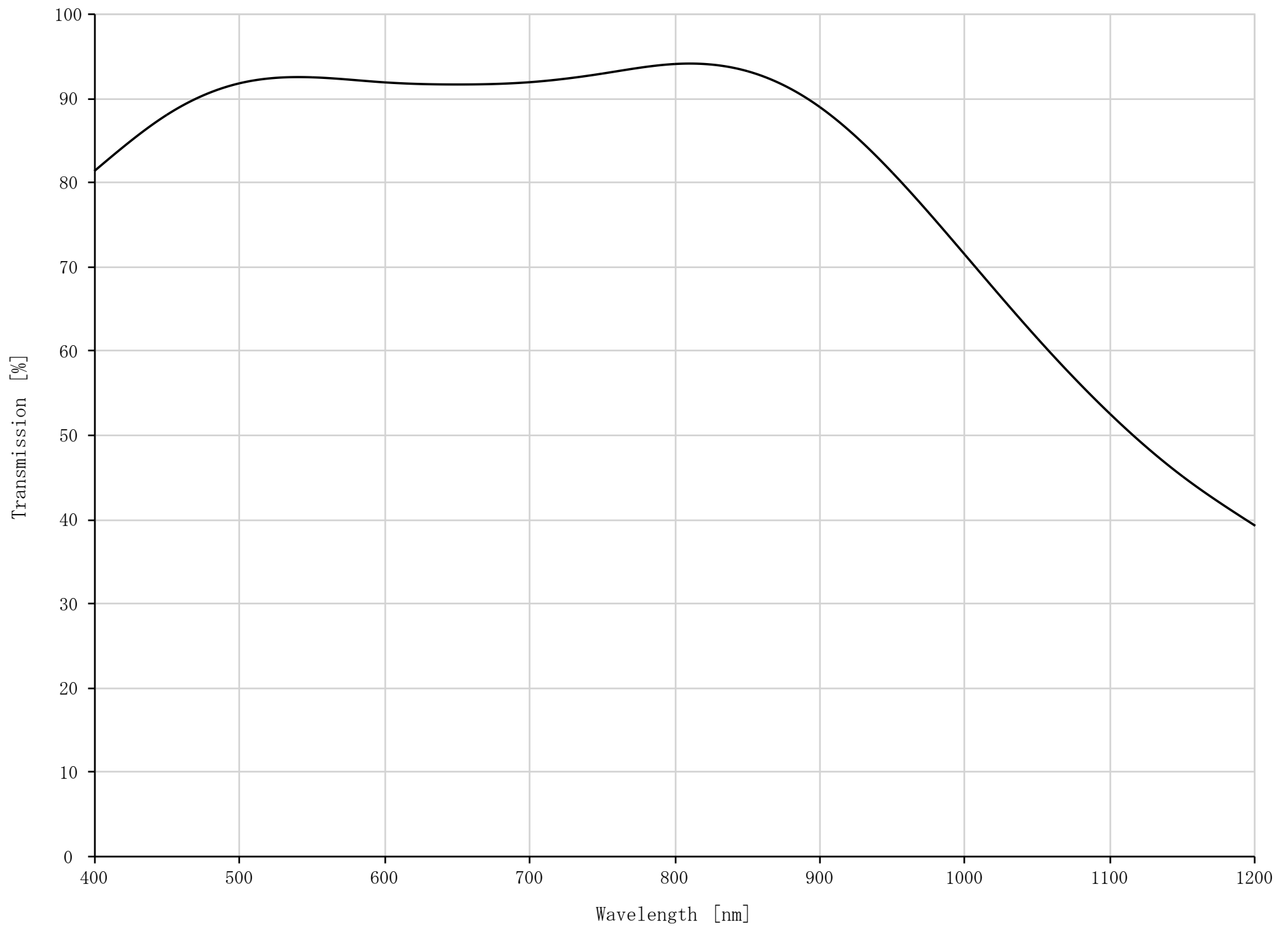
LM50FC Transmission
