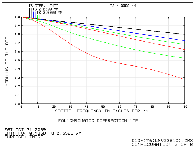
Iris dia. \phi 5.0 F2.8 Wide ( f=3.5\text{mm} )
