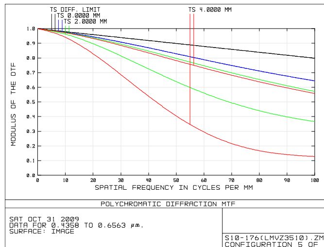
Iris dia. \phi 5.8 F2.8 Middle ( f=6.0\text{mm} )
