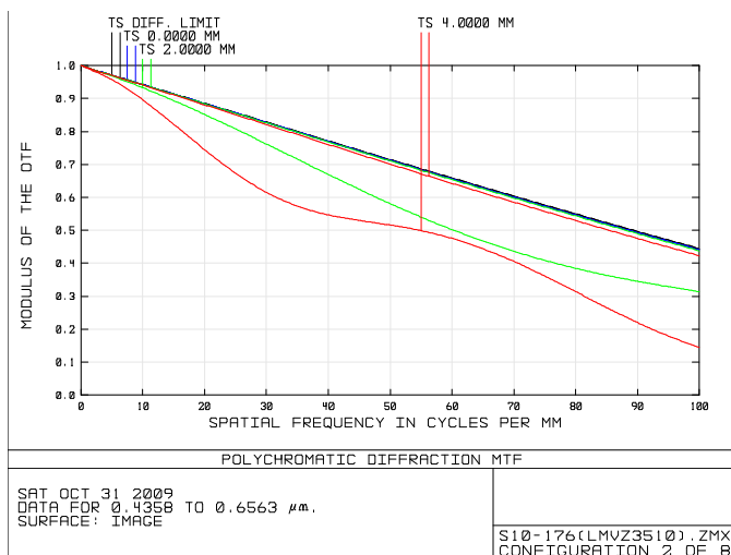
Iris dia. \phi 1.8 F8 Wide (f=3.5mm)
