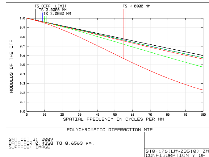
Iris dia. \phi 4 F5.6 Tele (f=9.8mm)
