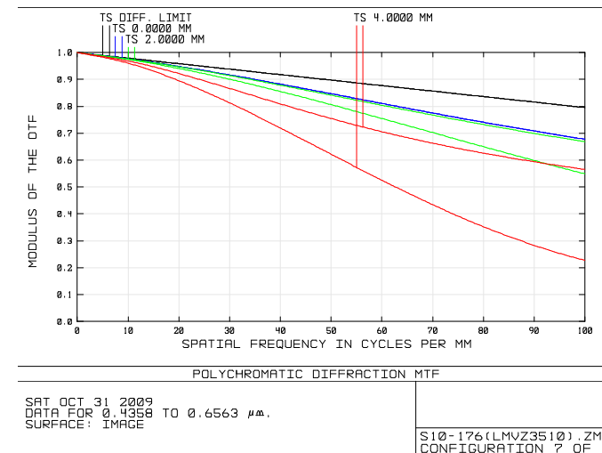
Iris dia. \phi 8.0 F2.8 Tele ( f=9.8\text{mm} )
