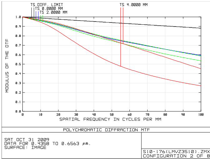
Iris dia. \phi 8.8 F1.6 Wide (f=3.5mm)
