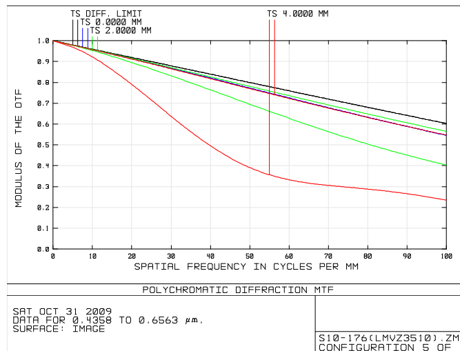
Iris dia. \phi 2.26 F5.6 Middle (f=6.0mm)
