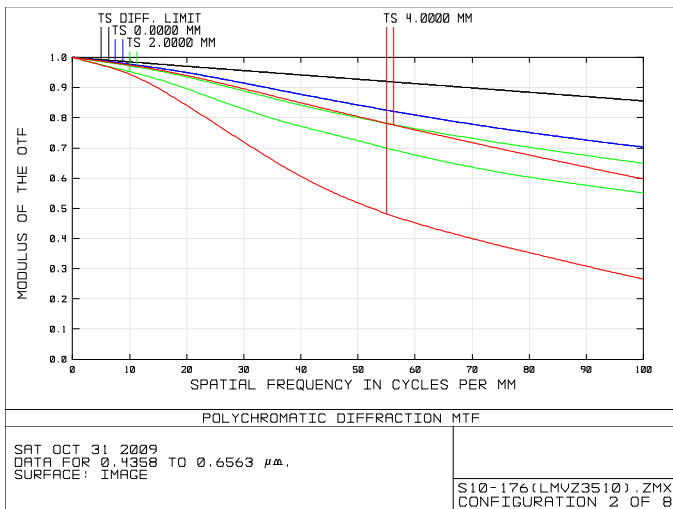
Iris dia. \phi 7.0 F2.0 Wide (f=3.5mm)
