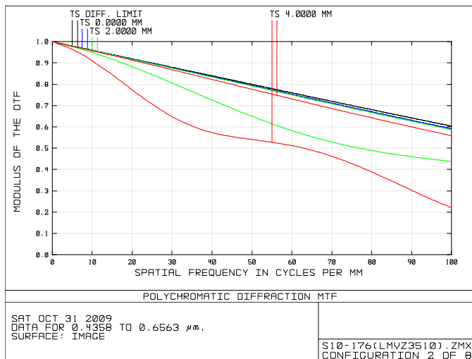
Iris dia. \phi 2.5 F5.6 Wide (f=3.5mm)
