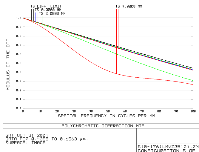
Iris dia. \phi 2.0 F9.4 Middle (f=6.0mm)
