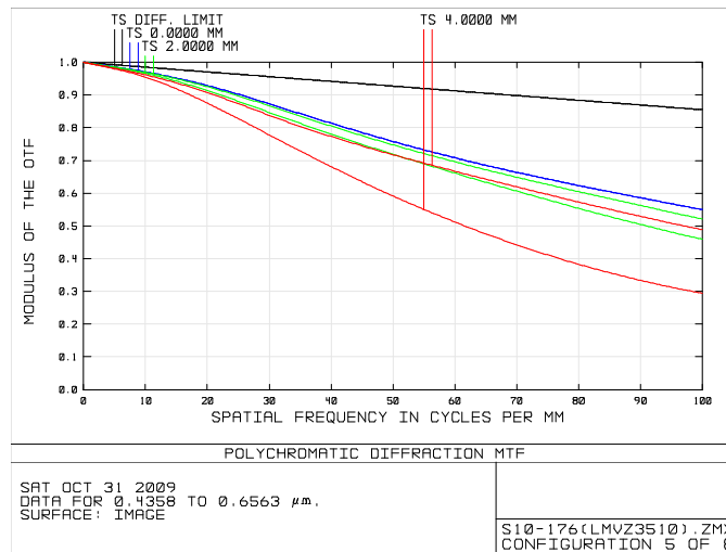
Iris dia. \phi 8.0 F2.0 Middle (f=6.0mm)
