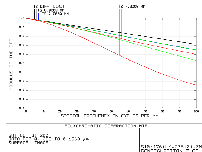
Iris dia. \phi 5.6 F4 Tele ( f=9.8\text{mm} )
